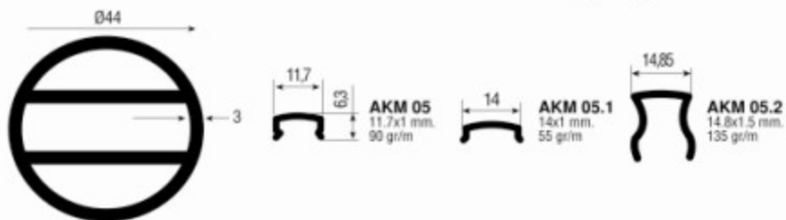
AKM 18.2 44x3 mm, 1623 gr/m
