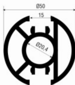
AKM 04.2 50x2.5 mm. 1730 gr/m
