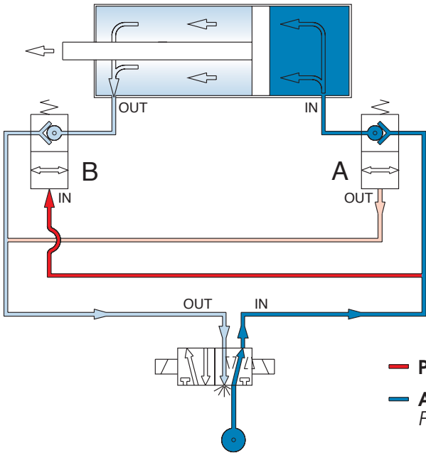
Cilindro in Movimento Cylinder in action
